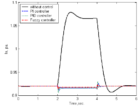
Figure (8): Speed-time response
