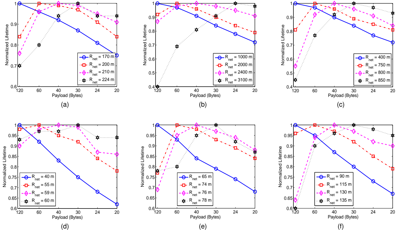
Fig. 4. Normalized lifetimes wrt. payload size for six different SG environments and power levels are optimized at link level for various sized (wrt. to R_{net} ) disk shaped random networks (a) OUS-L, (b) UNT-L, (c) IMP-L, (d) OUS-N, (e) UNT-N, and (f) IMP-N.
